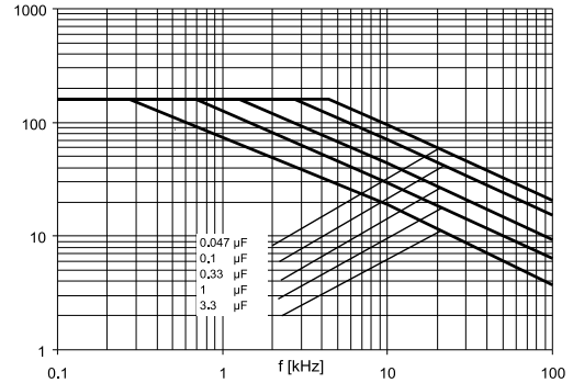
250 Vdc / 160 Vac
