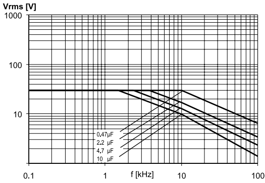
50 Vdc / 30 Vac
