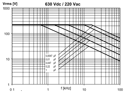
630 Vdc / 220 Vac
