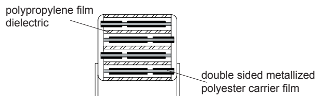
3 sections (700Vac)
