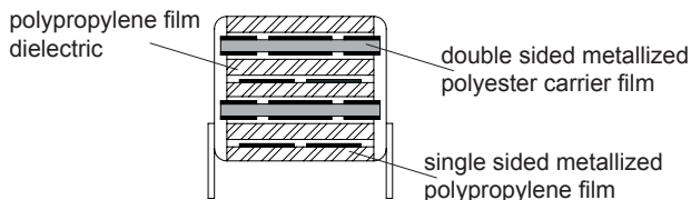
4 sections (900Vac)
