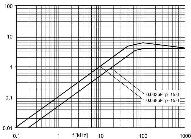
250 Vac
