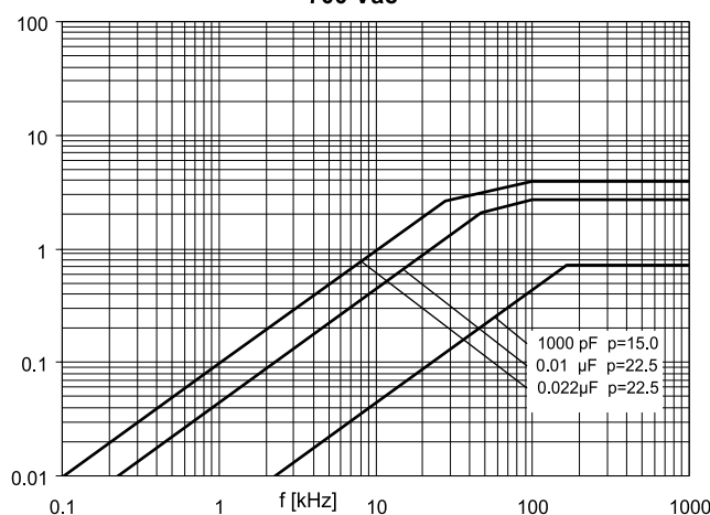
700 Vac
