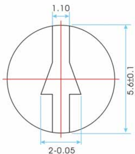
DETAIL B
